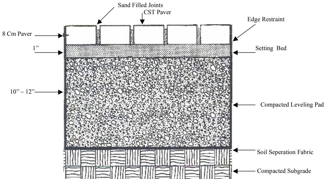
FIGURE C · Typical Heavy Construction Detail Roadway · Industrial/Heavy Truck · Gas Station
