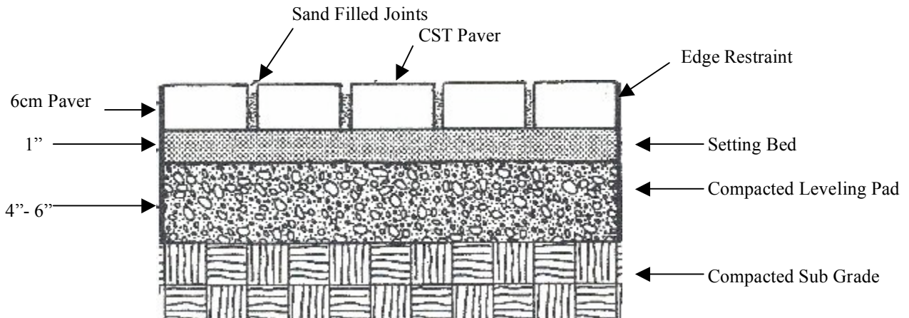
FIGURE B · Typical Light Vehicular Detail
